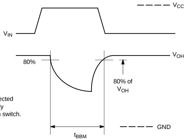
Figure 12. Break-Before-Make Time
