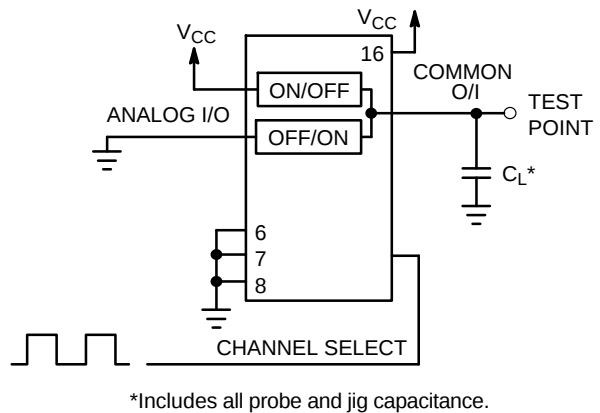
Figure 14. Propagation Delay, Test Set-Up Channel Select to Analog Out
